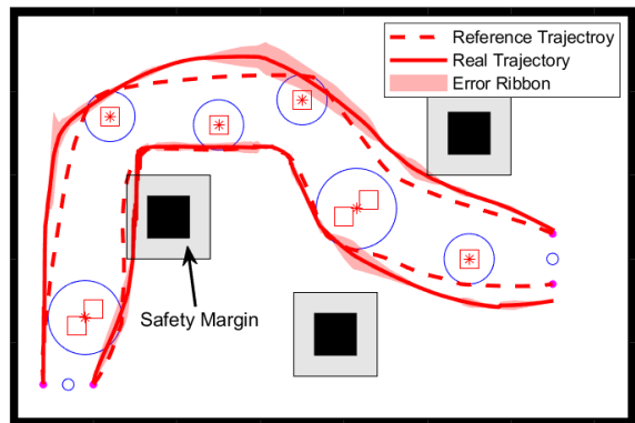
Fig. 8: Reference and tracked trajectories of the tethered robot duo. The red shadows indicate the variations of five executions.
