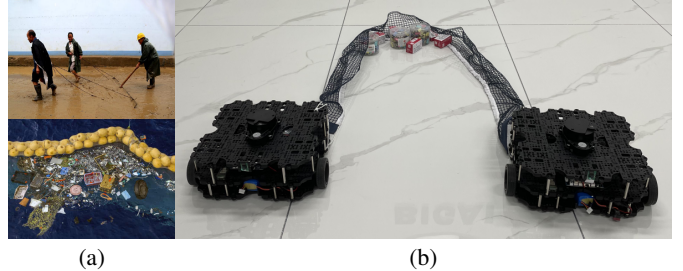
Fig. 1: (a) Two examples in daily life. Humans use long/flexible structures to gather scattered objects, a similar setup akin to the one proposed in our work (Source: online). (b) Two Wheeled Mobile Robots (WMRs) tethered by a net as a duo. Our framework cooperatively plans the robot duo's trajectories, indirectly maintaining the net's shape through motions. It also handles the uncertainty of the increasing payloads using Model Reference Adaptive Control (MRAC) to properly track the trajectories during operation.
