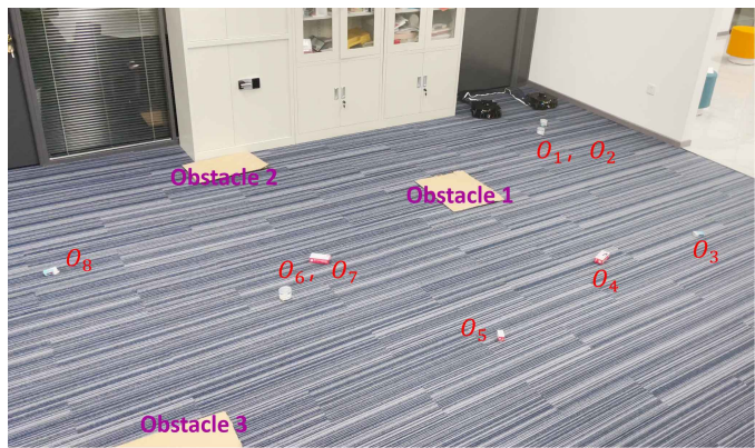
(a) Experimental environment. Eight objects are placed on the floor. The robot duo is tasked to gather them with a tethered net while avoiding obstacles during its navigation.
